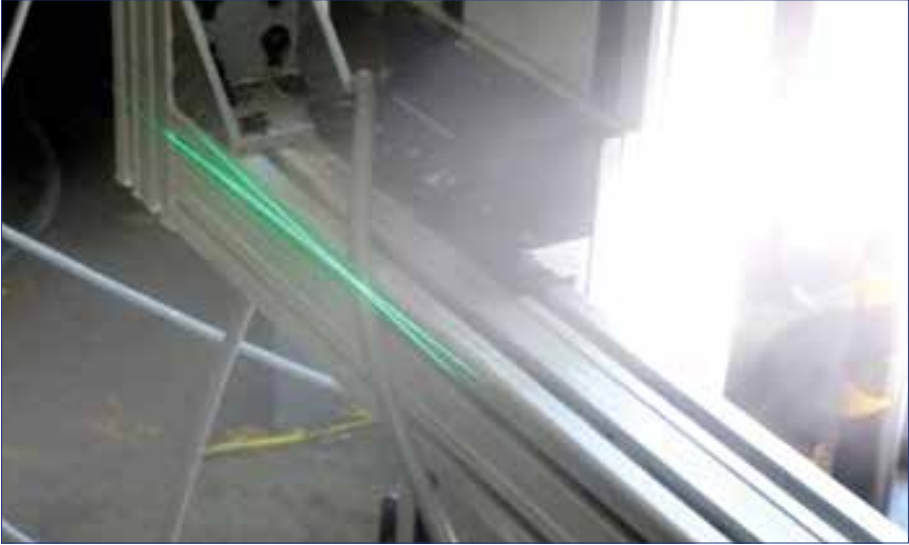
Figure 25. Phase Doppler Particle Analyzer showing spray through laser beams
