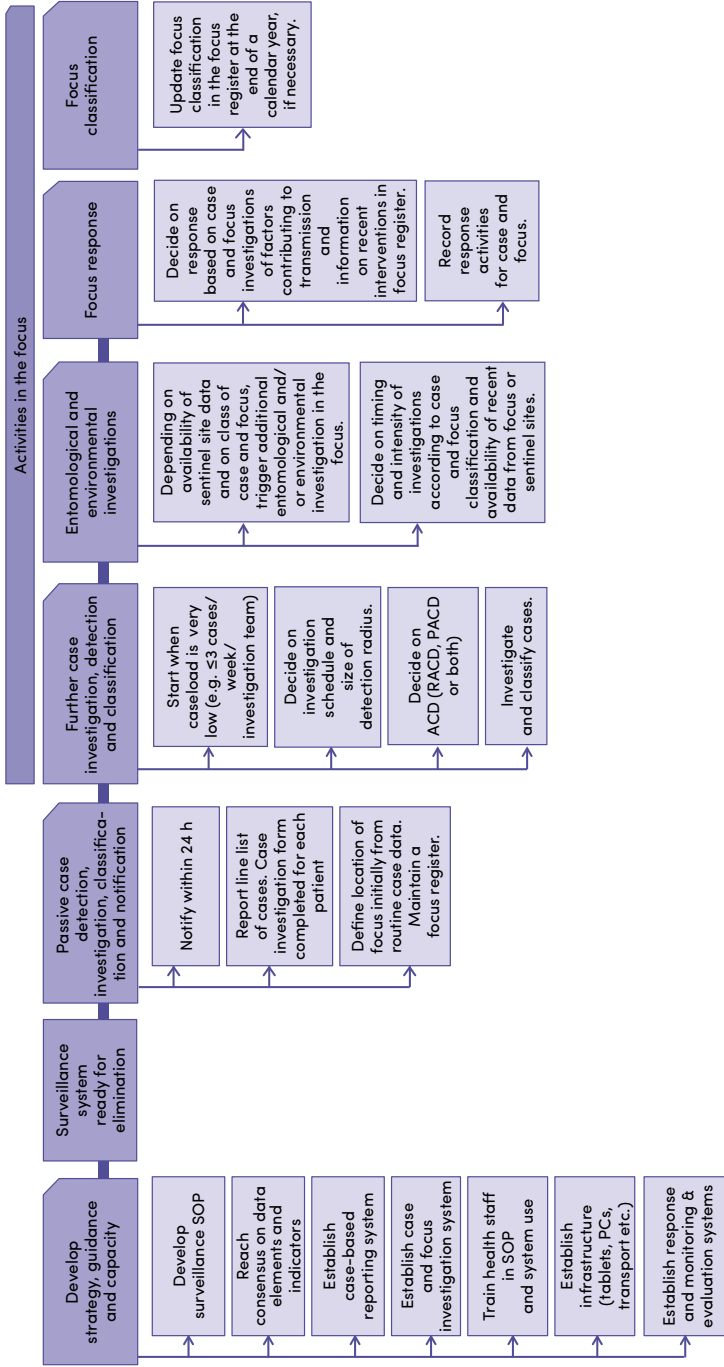
FIG. 6. Processes and activities for establishing malaria surveillance for elimination
