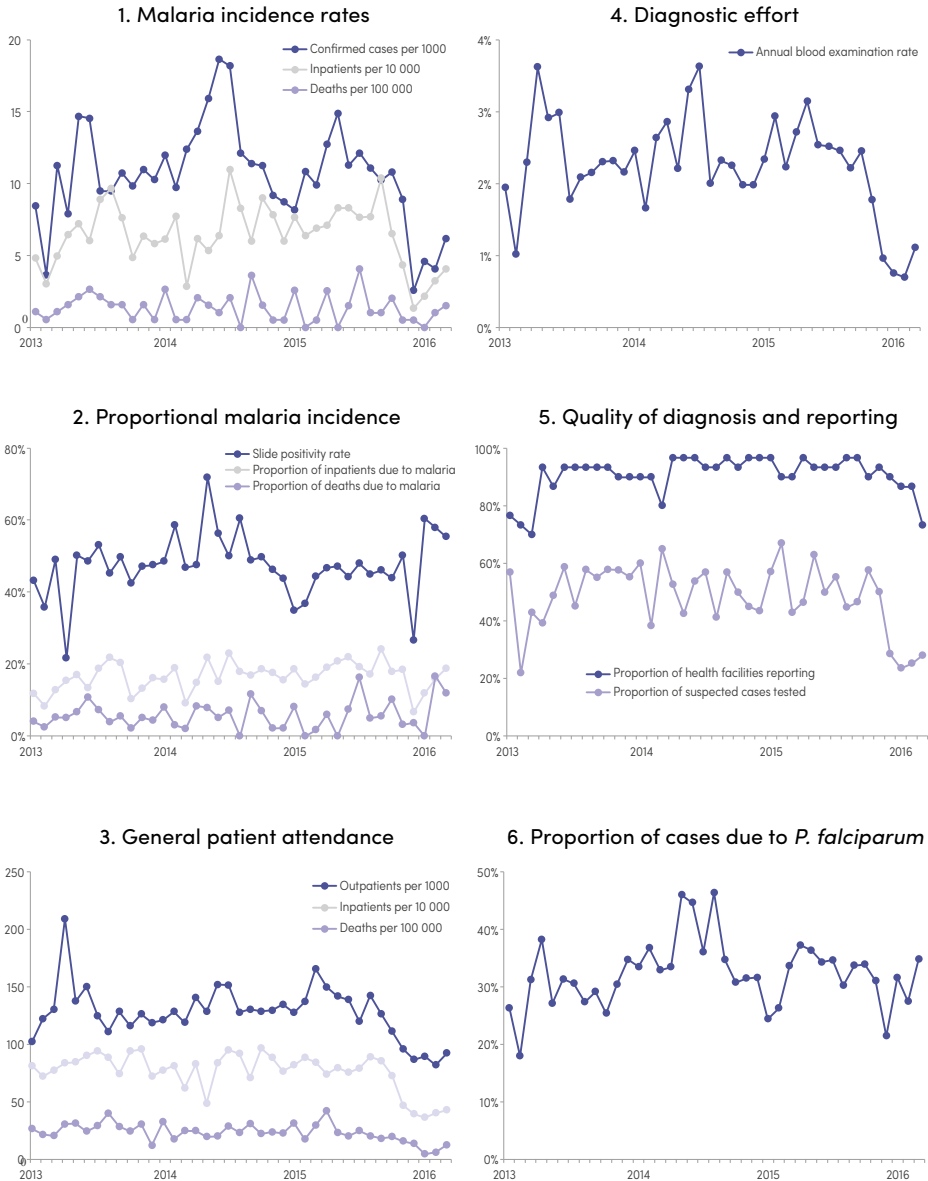
FIG. 26. Charts for analysis of malaria trends
